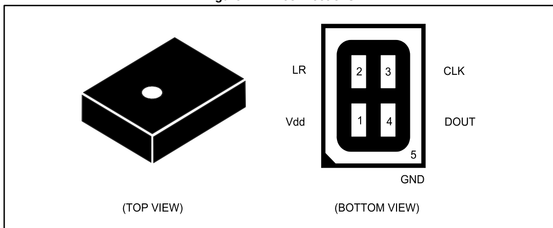
Figure 1: Pin connections
