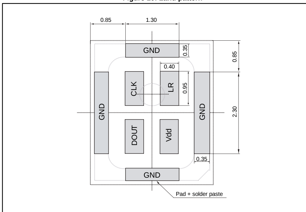
Figure 10: Land pattern
